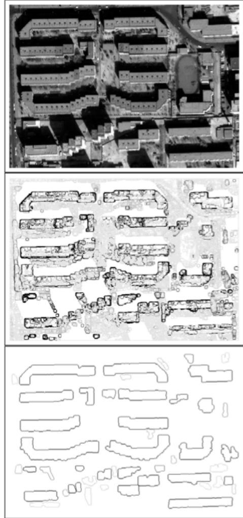
Fig. 1. Illustration of the cut-and-merge algorithm. Top: original image. Middle: superimposition of the contours extracted during the cut step; Bottom: building candidates resulting from the merge step. The grey level of the contours is inversely proportional to the probability to delineate a building-like object.
