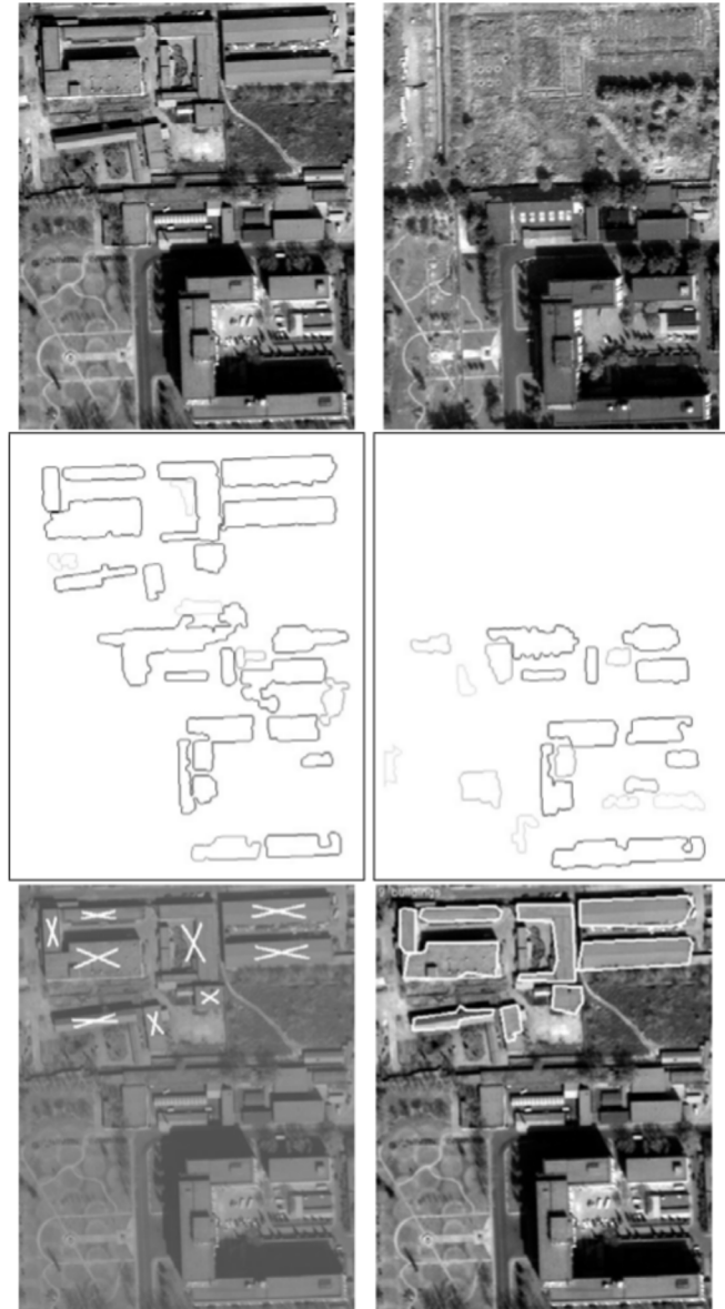
Fig. 2. Top: Original images. Center: candidate buildings' contours retrieved from cut-and-merge ; Bottom: building-object changes represented by polygonal approximation of the contours (right) or marked with a cross (left) –black for new building, white for disappeared.
