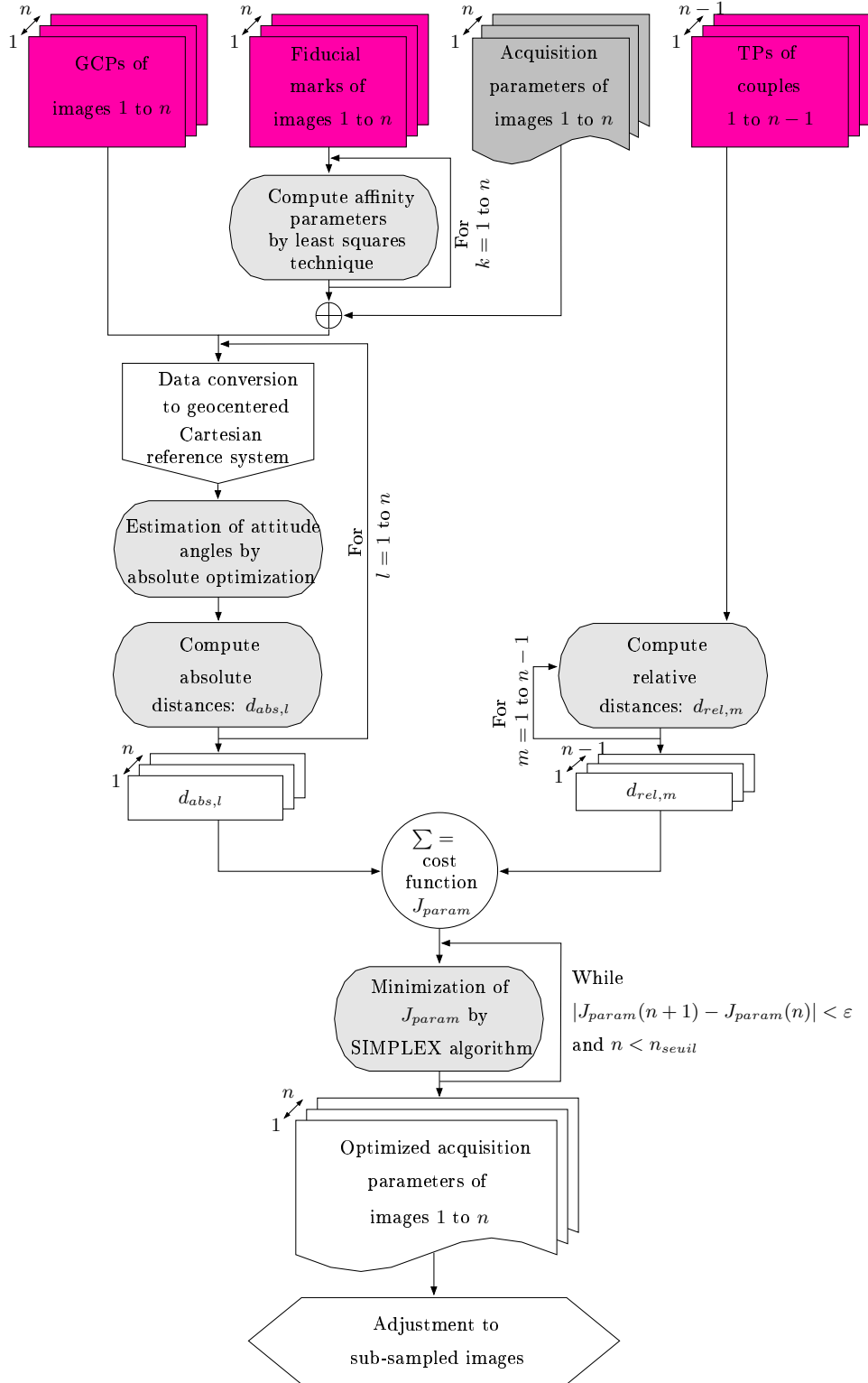
Figure 3.15: Algorithmic summary of the overall optimization of the image acquisition parameters with n aerial images.
