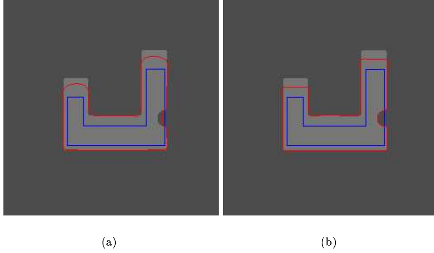
Figure 6.11: Segmentation with the Chan and Vese model and the shape constraint authorizing the parallel variations: (a) without quadratic correction and \lambda_{para} = 50 at instant n_0 ; (b) with quadratic correction, \lambda_{para} = 50 , \lambda_{quad} = 7 and a = 0.5 .
