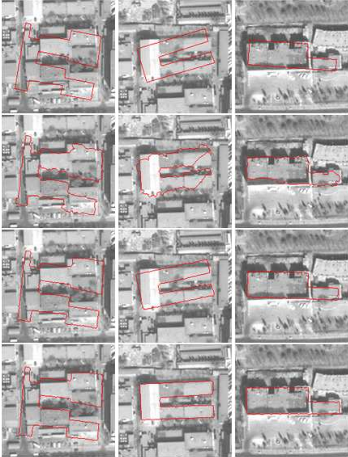
Figure 5.24: Spatio-temporal variation of lambda with the GVF model and \lambda_{min} = 1 , \lambda_{max} = 5 , d_0 = 5 :
