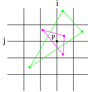
Figure 3.20: Projection of a triangle of the epipolar DSM to the orthoscopic grid.
