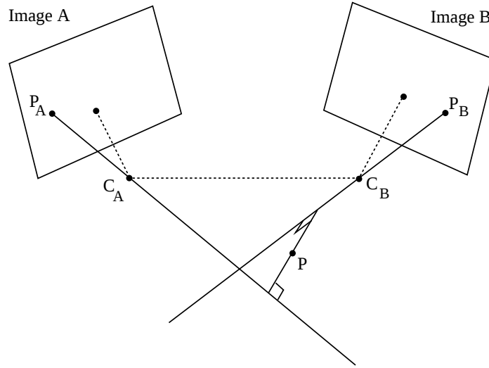
Figure 3.3: For two conjugated points P_A and P_B , the relative orientation makes it possible to calculate the position of point P in the coordinates system linked to the pair of images. P is defined as the center of the smallest segment joining the straight lines (P_A, C_A) and (P_B, C_B) .
