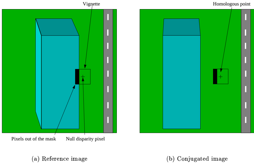
Figure 3.9: Application of the mask on the context vignette. The part of the building is withdrawn from the correlation window thanks to the mask adaptive geometry. The homologous pixel is found.
