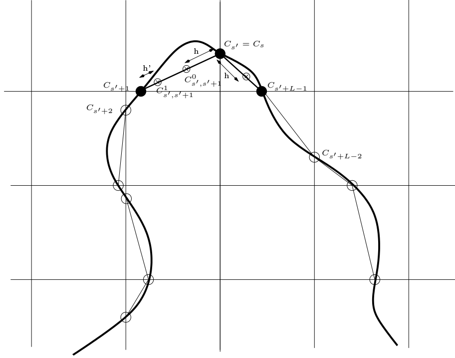
Figure 6.4: Diagram describing the sampling mode with a Bessel function for profile \Psi
