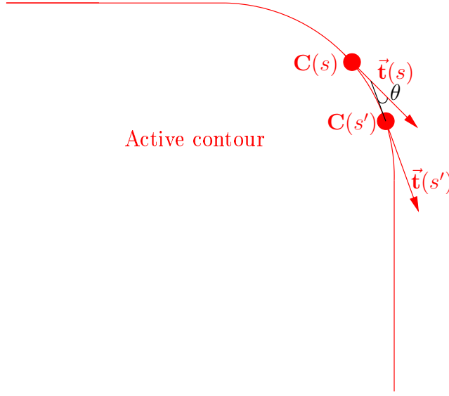
Figure 6.2: Long-range interaction due to the corrective quadratic energy. The tangents \vec{t}(s) and \vec{t}(s') will tend to be orthogonal or collinear.
