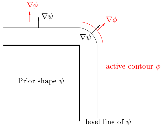
Figure 6.1: Rounding effect at geometrical singularities due to the new shape constraint energy based on normals alignment
