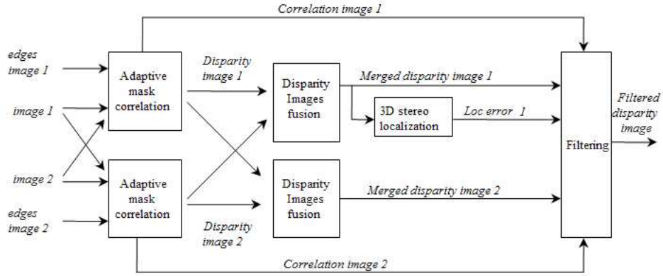
Figure 3.11: Summary of the 3D reconstruction process.
