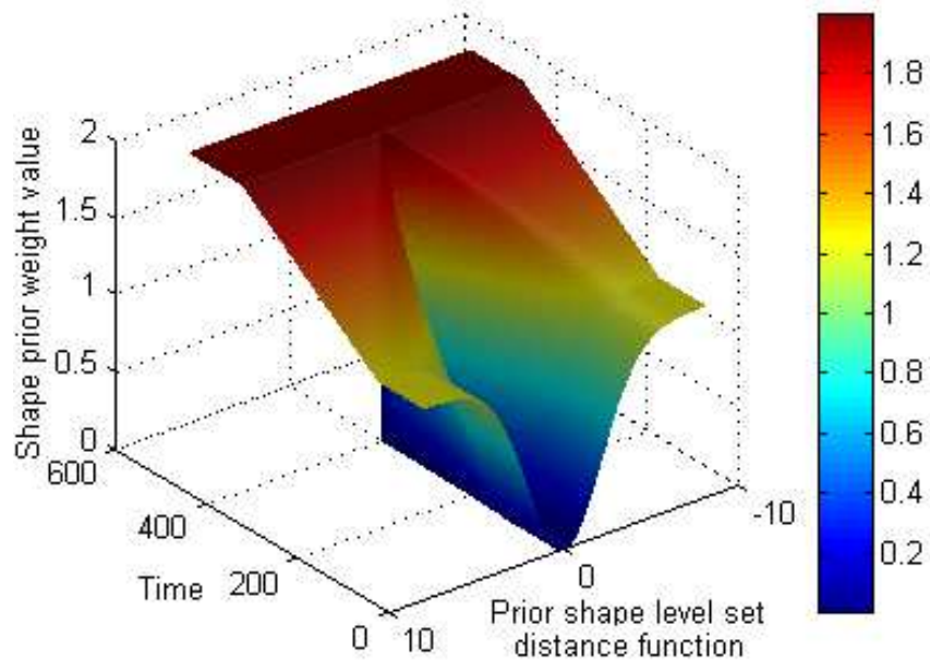
Figure 5.2: Spatio-temporal variation of the function weighting the shape constraint. d_0 = 3 , t_1 = 100 , t_2 = 400 , \lambda_{min} = 1.25 and \lambda_{max} = 2 .
