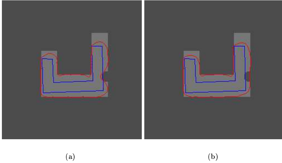
Figure 6.9: Segmentation with shape constraint authorizing parallel variations: (a) \lambda_{para} = 15 ; (b) \lambda_{para} = 30
