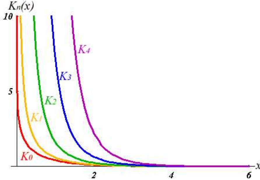
Figure 6.3: Modified Bessel functions of the second kind.
