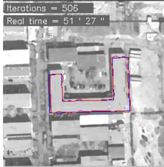
Figure 6.13: Experiment with a real image, the prior shape is the result of the matching with the conventional shape constraint. The segmentation is carried out with the Chan and Vese model, the shape constraint authorizing the parallel variations and with quadratic correction \lambda_{para} = 4 , \lambda_{quad} = 0.5 and a = 0.5 .
