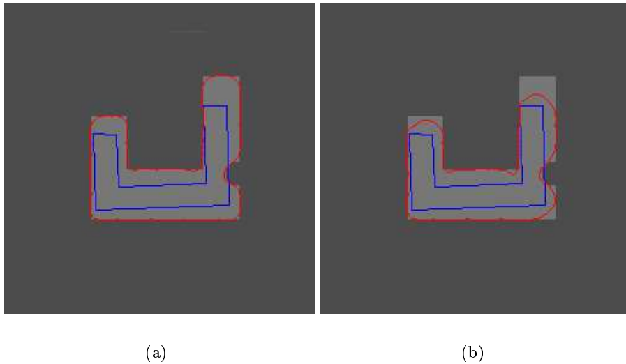
Figure 6.8: Segmentation with shape constraint authorizing parallel variations: (a) \lambda_{para} = 5 ; (b) \lambda_{para} = 10
