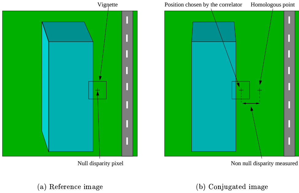
Figure 3.8: Error in the case of occluded zones with a fixed correlation window. (a) a null disparity pixel is considered. (b) its homologous point in the conjugated image is not found because part of the building is taken into account in the correlation window.
